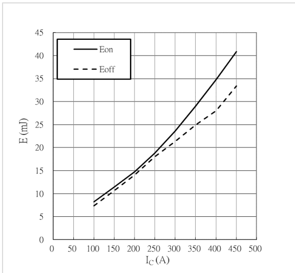
Switching losses IGBT, Inverter V_{GE} = +15\text{ V} / -8\text{ V} , R_{GON} = 2.0\ \Omega , R_{Goff} = 2.0\ \Omega , V_{CE} = 600\text{V} , T_j = 25^\circ\text{C}
